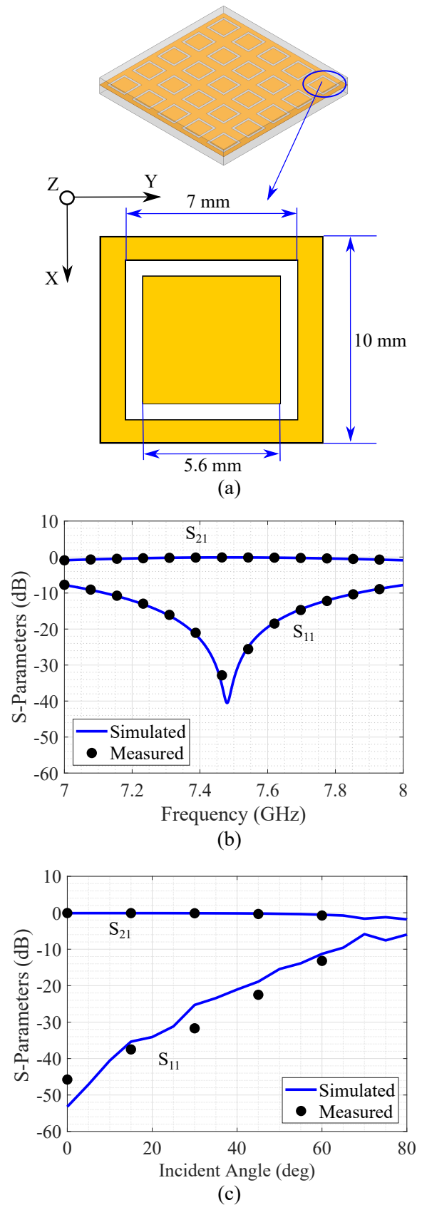
Fig. 3. Frequency Selective surfaces (FSS). (a) Design schematic. (b) Simulated and measured S -parameters in frequency domain. (c) Simulated and measured S -parameters in angle domain.
